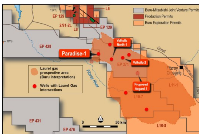
Paradise-1 Interpreted Valhalla Laurel Formation Accumulation
